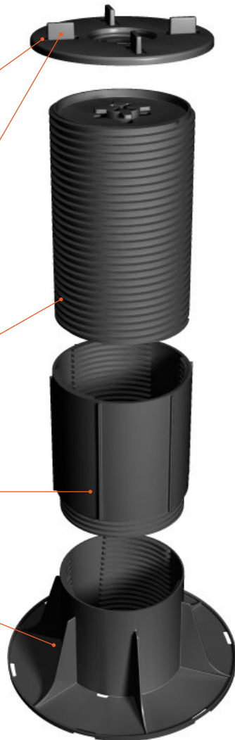
BRSP 3mm rubber shock pad for pedestal base part no: 50.1001
