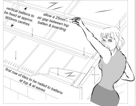
Boarded Roof Application
