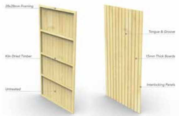
Pre-cut external timber cladding panels for quick and easy assembly.
