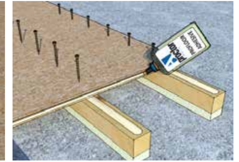
Fig. 12 Concrete Installation
