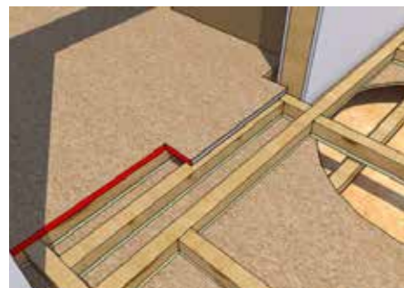
Fig. 16 Timber Installation
